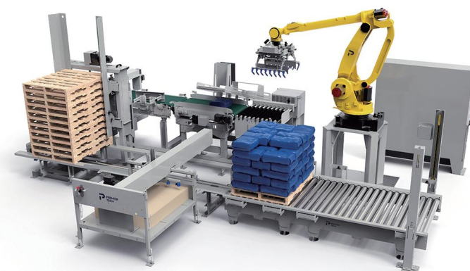
● Palletizing Machine
